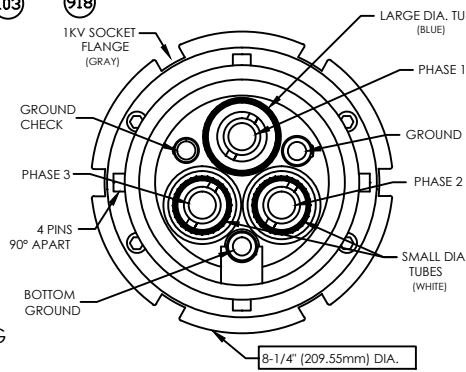
CONTACT END VIEW
